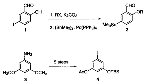
Scheme 1. Preparation of 'A-ring' and 'B-ring'.
