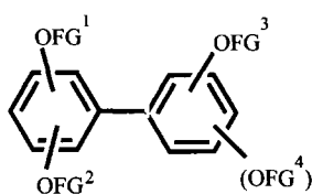
Figure 2. Generic structure of the biphenyl library.
