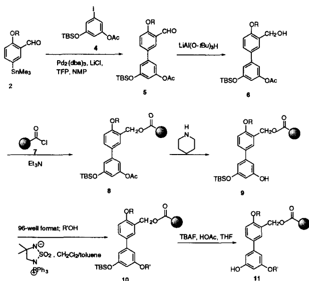
Scheme 2. Preparation of biphenyl products.
